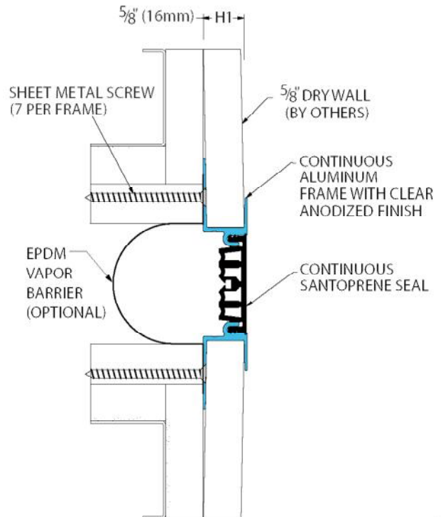
112-A07 Wall/Wall Ceiling/Ceiling with Vapor Barrier (2" (50mm) system shown)
