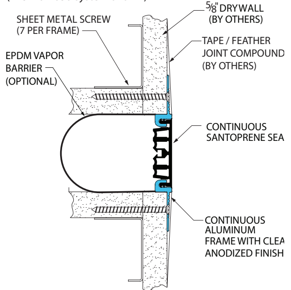
EPDM Vapor Barrier (113-A07-050 system shown)
