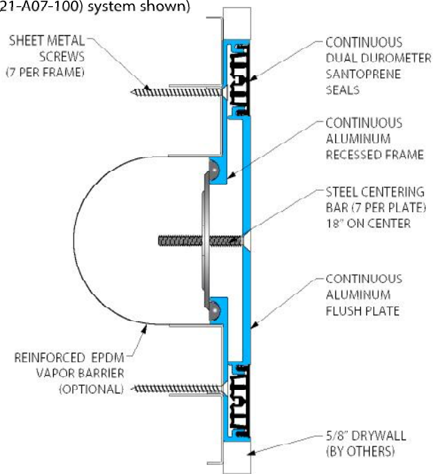
Vapor Barrier System (4" (221-A07-100) system shown)
