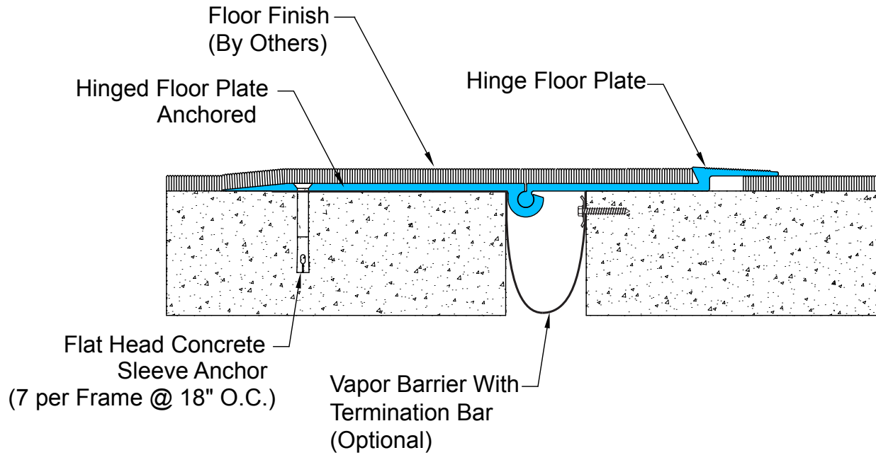
807-A01 Floor/Floor With Vapor Barrier (2" (51mm) system shown)
