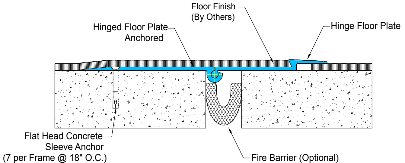
807-A01 Floor/Floor With Fire Barrier (2" (51mm) system shown)
