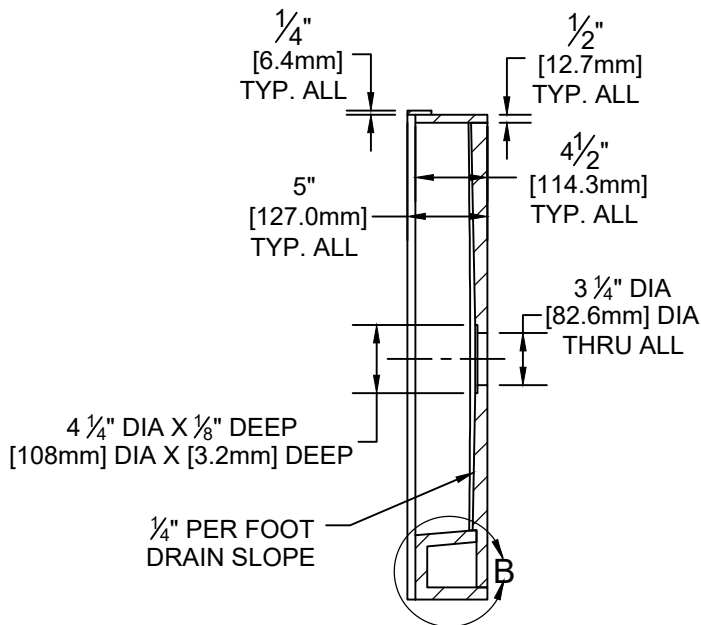
SECTION A-A LEFT OPENING SHOWN, RIGHT OPENING OPPOSITE
