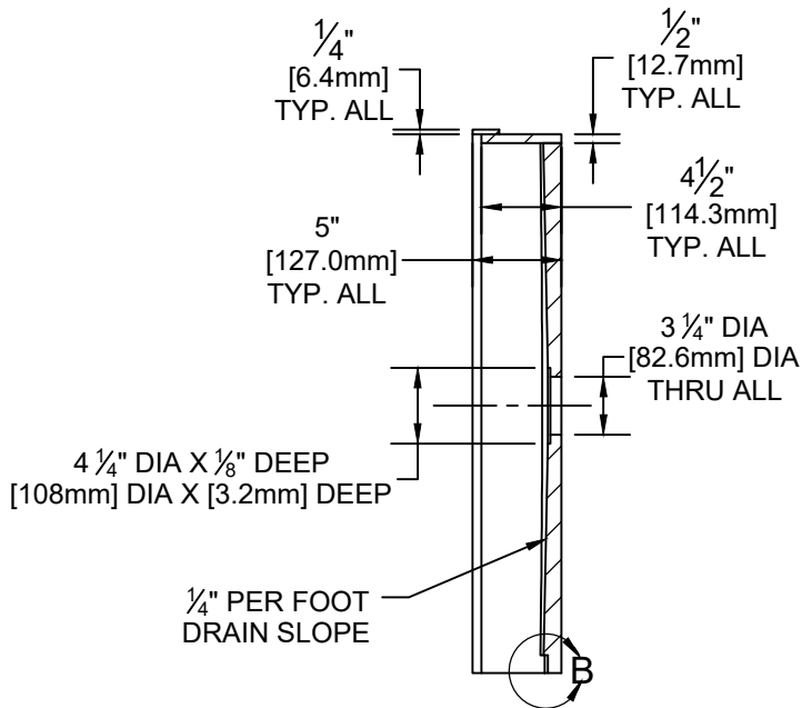
SECTION A-A LEFT OPENING SHOWN, RIGHT OPENING OPPOSITE
