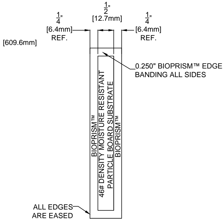
SECTION Z-Z NTS
